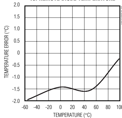
MAX1099 TEMPERATURE ERROR vs. REMOTE DIODE TEMPERATURE
